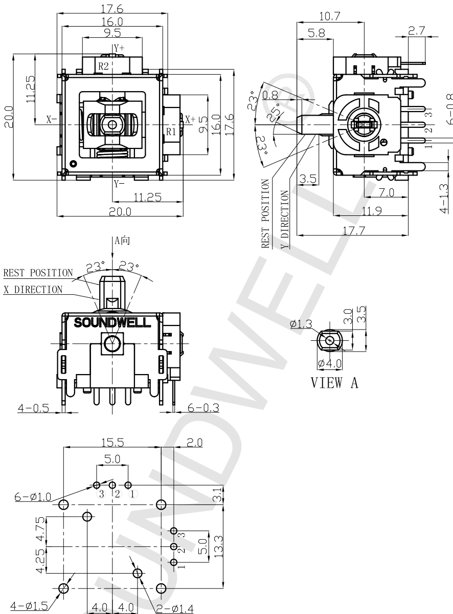
P. C. B MOUNTING HOLE DETAIL
